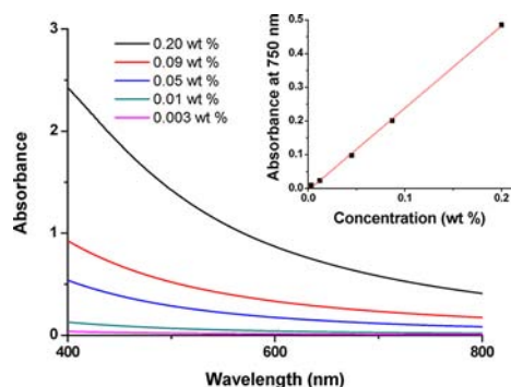
Figure 5. Visible absorption spectra for cross-linked polymersome dispersions at various concentrations. An arbitrary wavelength (750 nm) was used to construct a linear calibration plot (inset), allowing the concentration of non-adsorbed polymersomes remaining in the aqueous phase after emulsification to be determined via turbidimetry.
