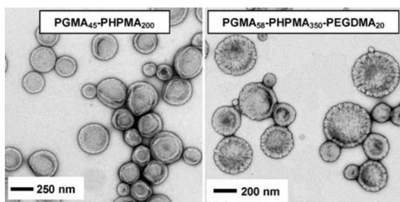
Figure 2. TEM images obtained for linear PGMA 45 -PHPMA 200 and cross-linked PGMA 58 -PHPMA 350 -PEGDMA 20 polymersomes.
