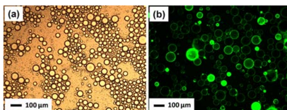
Figure 3. (a) OM image obtained for an n -dodecane-in-water Pickering emulsion prepared using PGMA 58 -PHPMA 350 -PEGDMA 20 cross-linked polymersomes. (b) Fluorescence microscopy image of the corresponding Pickering emulsion prepared using the equivalent fluorescein-labeled PGMA 58 -PHPMA 350 -PEGDMA 20 polymersomes.
